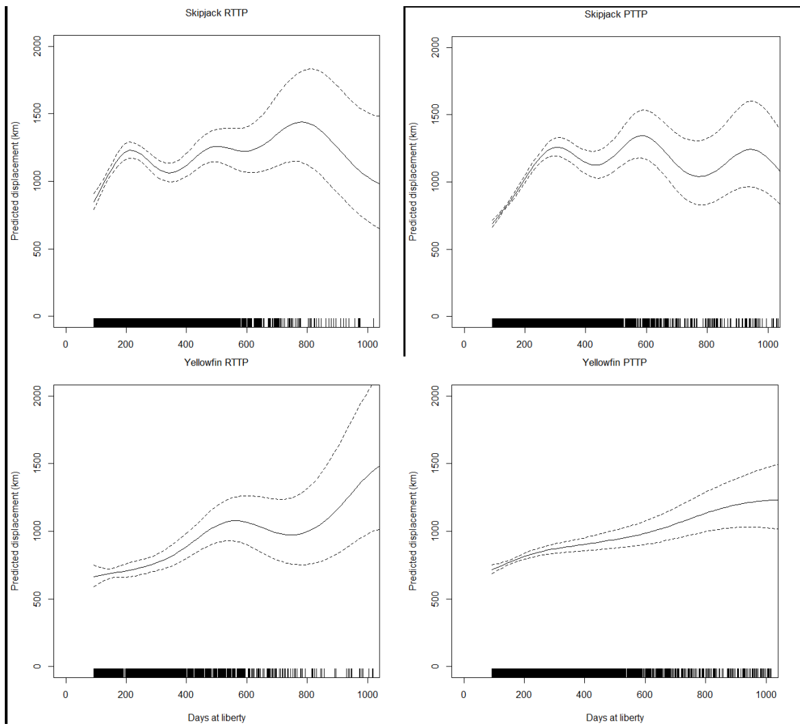
Figure 23: : Plots of median displacement by time estimated by GAMs, for the RTPP (left) and the PTTP (right) and for skipjack (above) and yellowfin (below) tunas. Predictions are for an average length recaptured fish (47cm RTPP and 44cm PTTP skipjack; 43cm yellowfin) released at 150E, 0N. The dotted lines represent 95% confidence intervals, and the 'rug' on the x axis marks values of the input data.
