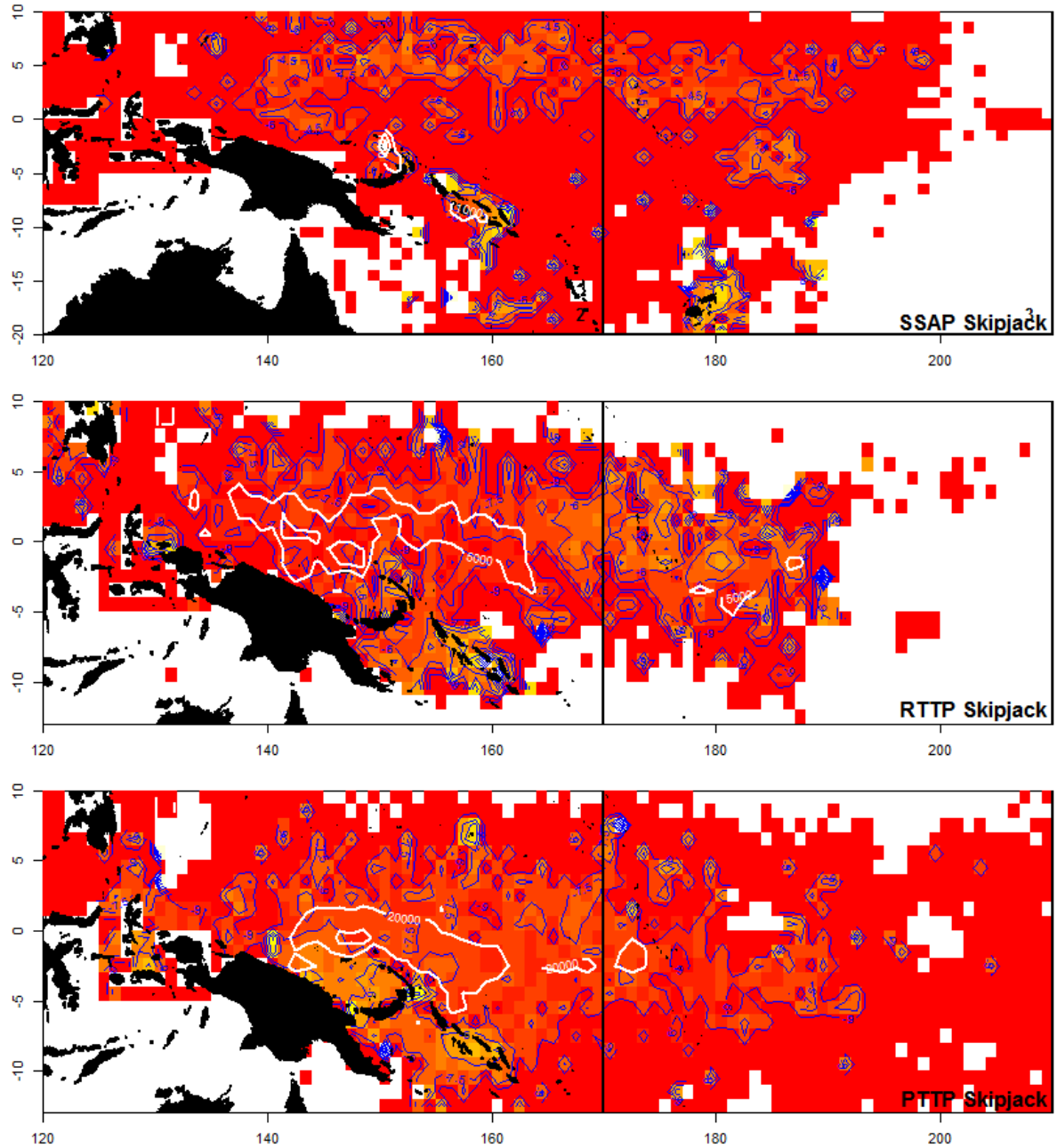
Figure 37: Tag recovery density map per 1 degree square for skipjack in the SSAP (top), RTP (middle) and PTP (bottom), for tags recovered after > 91 days (the mixing period). Yellow indicates higher tag density, and responses are on the log scale, so that density increases by a multiple of 4.5 with each blue contour line. The white contour lines indicate the areas of greatest purse seine catch.
